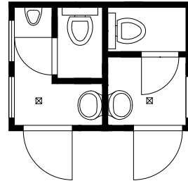
10f WC-Container Damen/Herren 2.990 x 2.435 x 2.800mm
