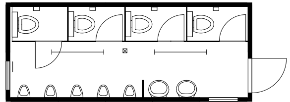
20f WC-Container Herren 6.055 x 2.435 x 2.800mm
